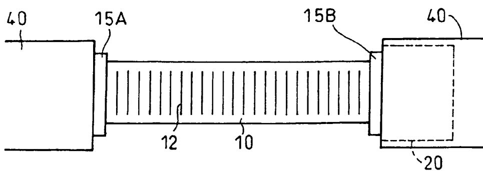
Fig. 3(2) Prior Art
